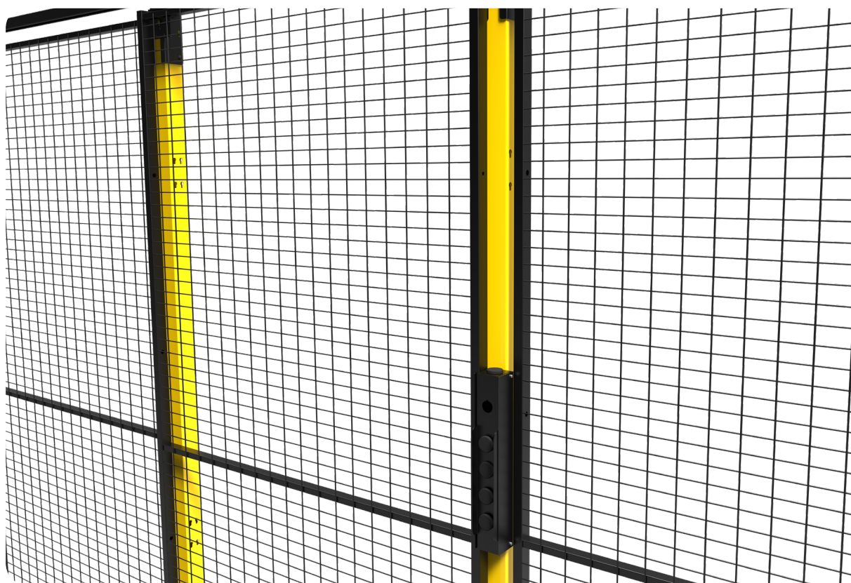
Push button enclosure mounted on post by sliding door.
